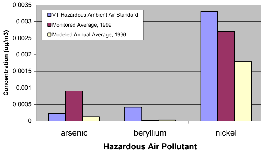
Comparison of 1996 NATA Modeled Concentrations with Vermont Ambient Monitoring Data (Burlington, VT)
